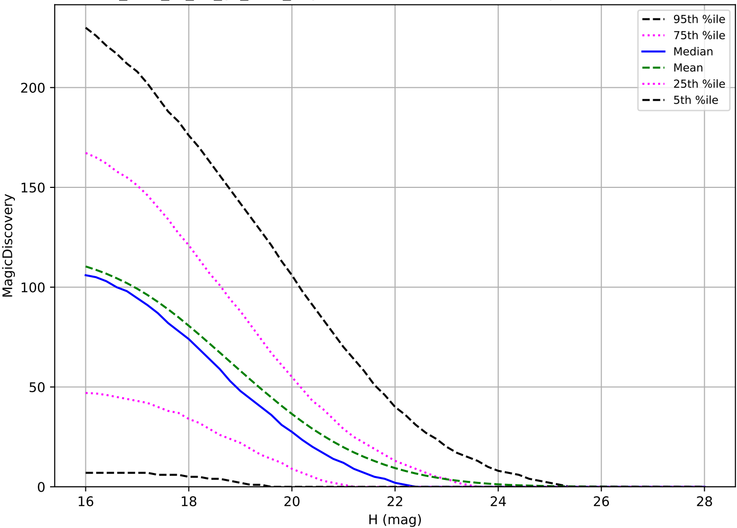
too_elab_r8_d2_gz_v3.4_10yrs: PHA 6 detections in 60 nights detection loss
