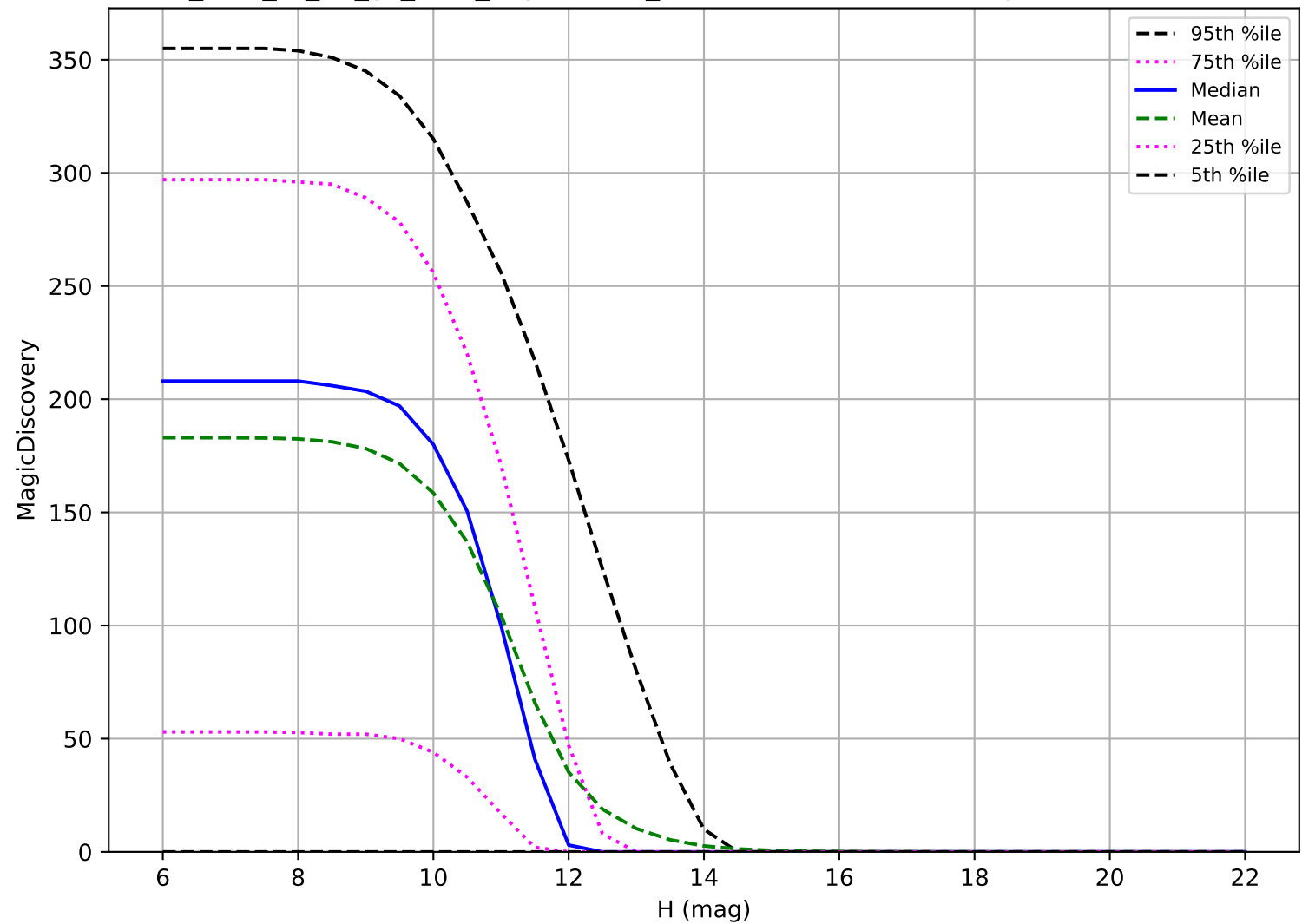
too_elab_r8_d2_gz_v3.4_10yrs: OCC_r20 6 detections in 60 nights detection loss
