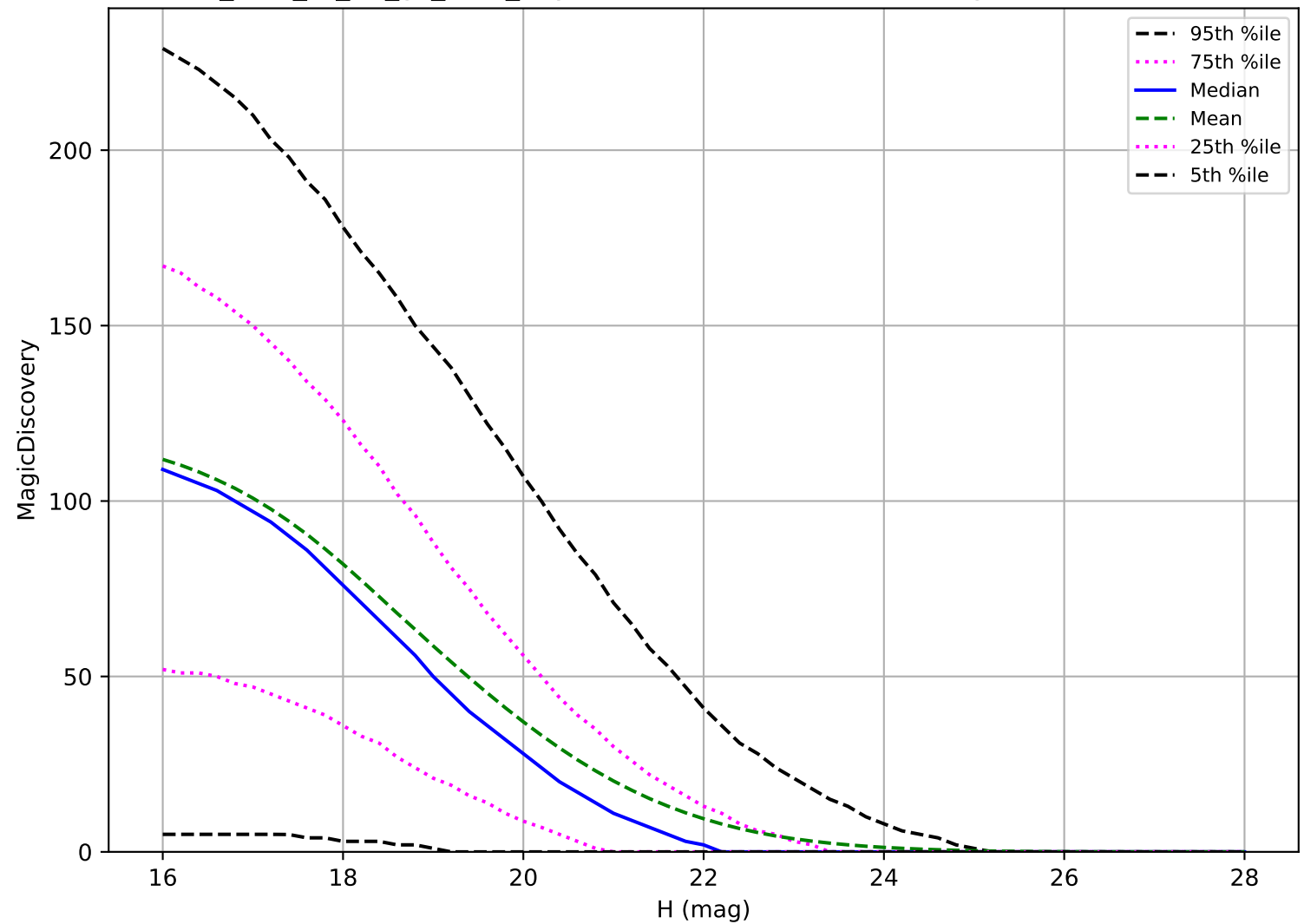
too_elab_r8_d2_gz_v3.4_10yrs: NEO 6 detections in 60 nights detection loss
