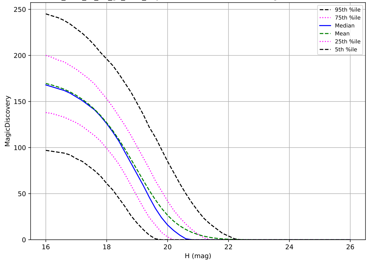
too_elab_r8_d2_gz_v3.4_10yrs: MBA 6 detections in 60 nights detection loss
