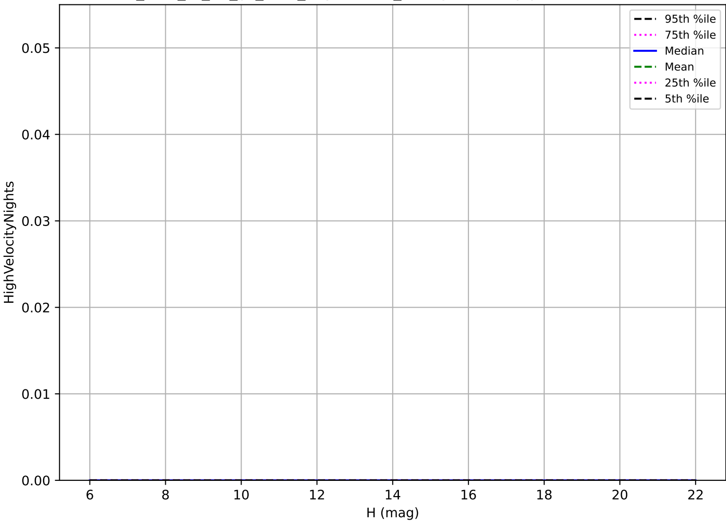
too_elab_r8_d2_gz_v3.4_10yrs: OCC_r5 High velocity pair detection loss
