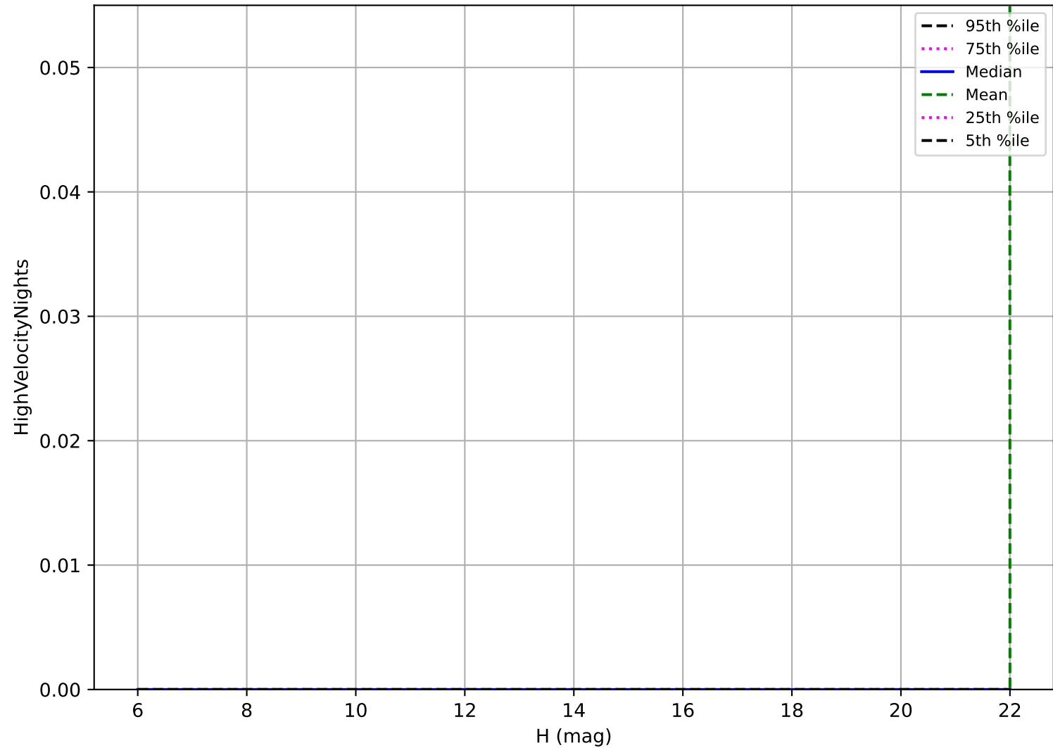
too_elab_r8_d2_gz_v3.4_10yrs: OCC_r20 High velocity pair detection loss
