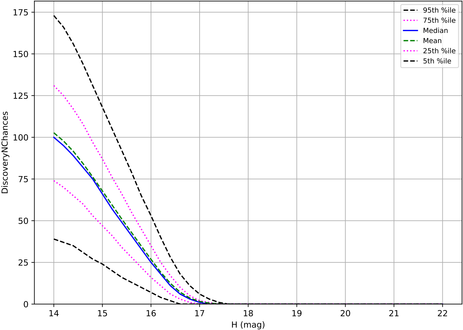
too_elab_r8_d2_gz_v3.4_10yrs: Trojan 3 pairs in 15 nights detection loss
