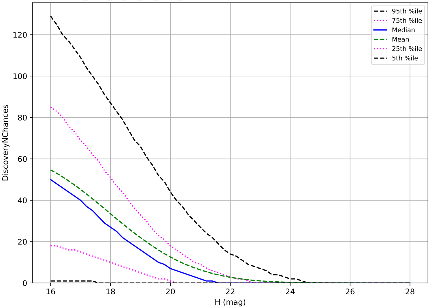
too_elab_r8_d2_gz_v3.4_10yrs: PHA 3 pairs in 15 nights detection loss
