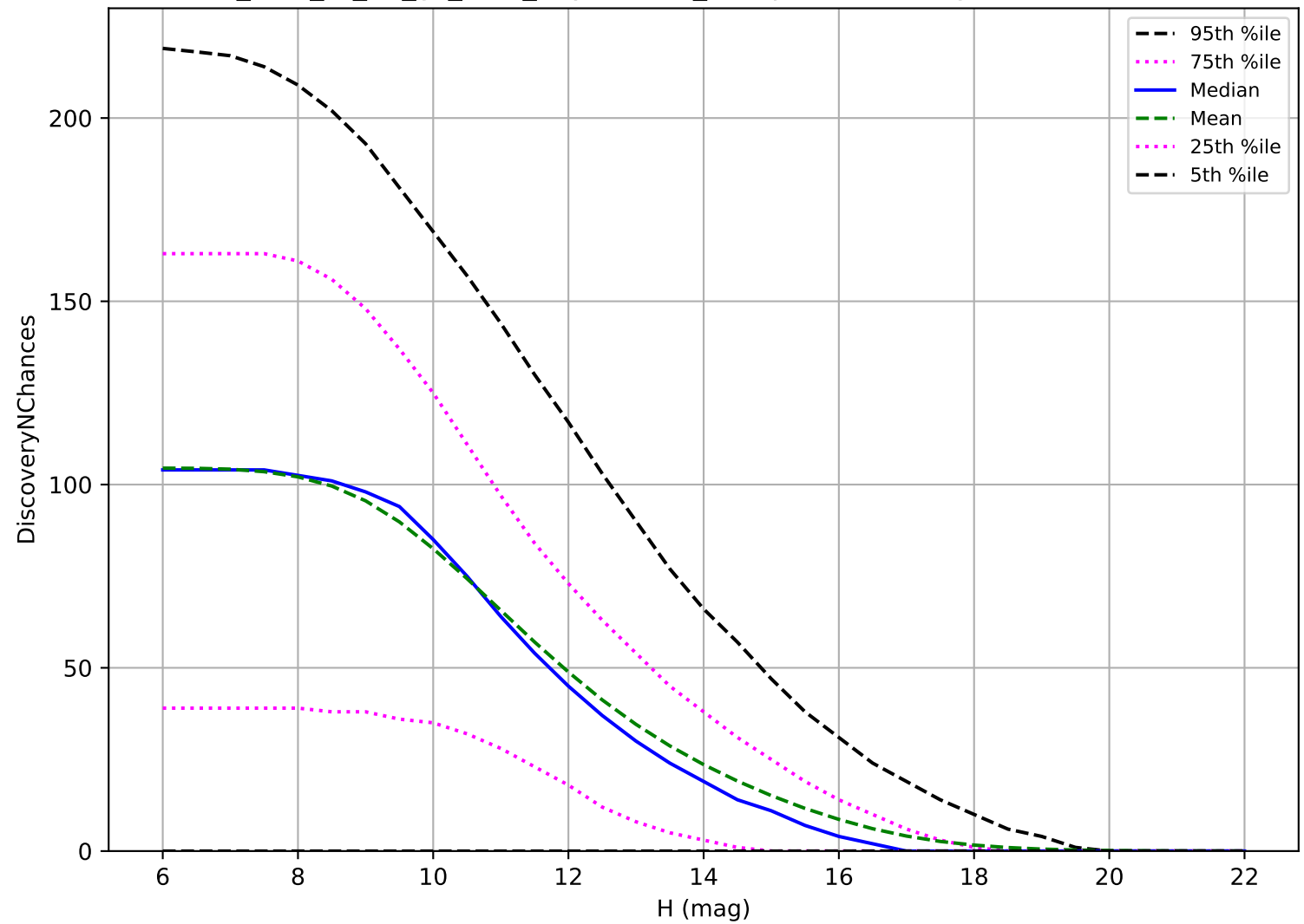
too_elab_r8_d2_gz_v3.4_10yrs: OCC_r5 3 pairs in 15 nights detection loss
