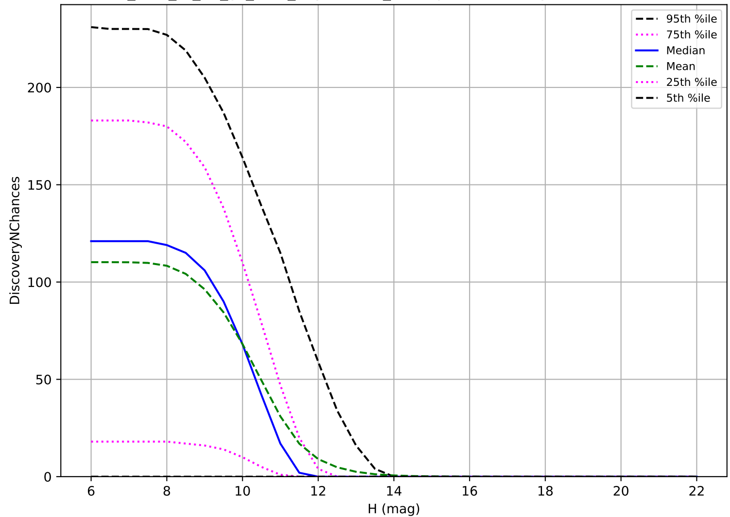
too_elab_r8_d2_gz_v3.4_10yrs: OCC_r20 3 pairs in 15 nights detection loss
