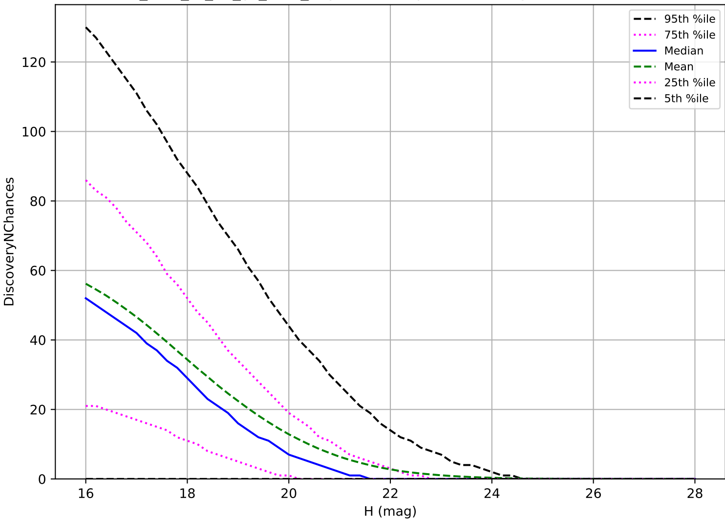
too_elab_r8_d2_gz_v3.4_10yrs: NEO 3 pairs in 15 nights detection loss
