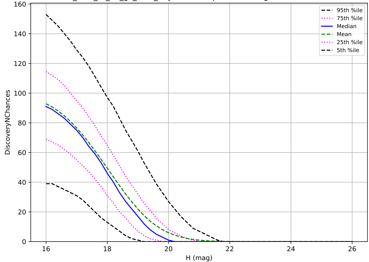
too_elab_r8_d2_gz_v3.4_10yrs: MBA 3 pairs in 15 nights detection loss
