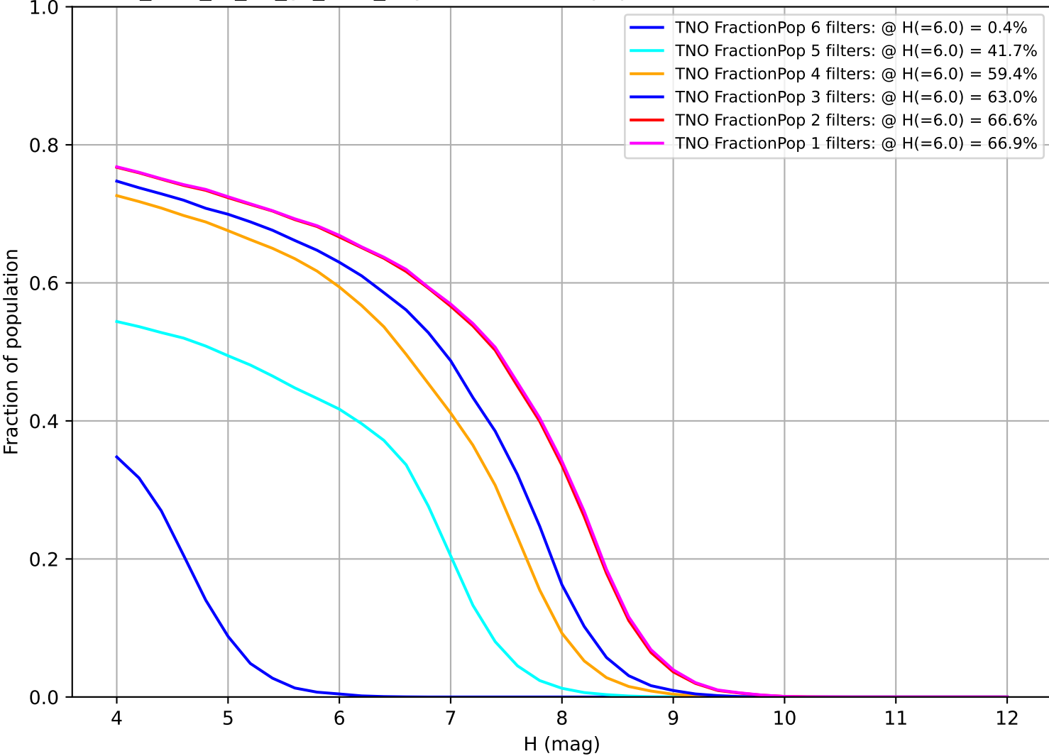
too_elab_r8_d2_gz_v3.4_10yrs: Fraction of population with colors in X filters TNO
