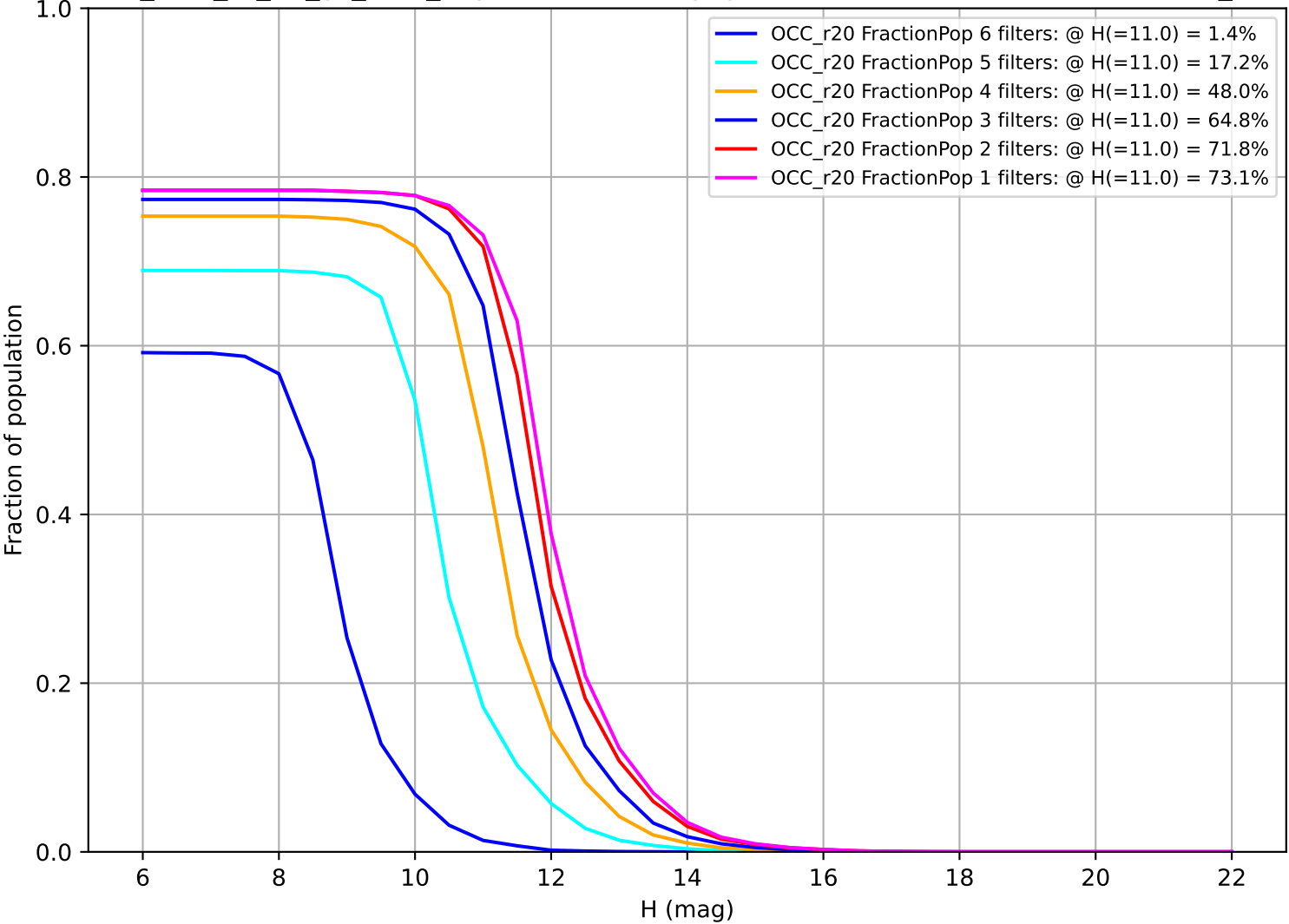
too_elab_r8_d2_gz_v3.4_10yrs: Fraction of population with colors in X filters OCC_r20
