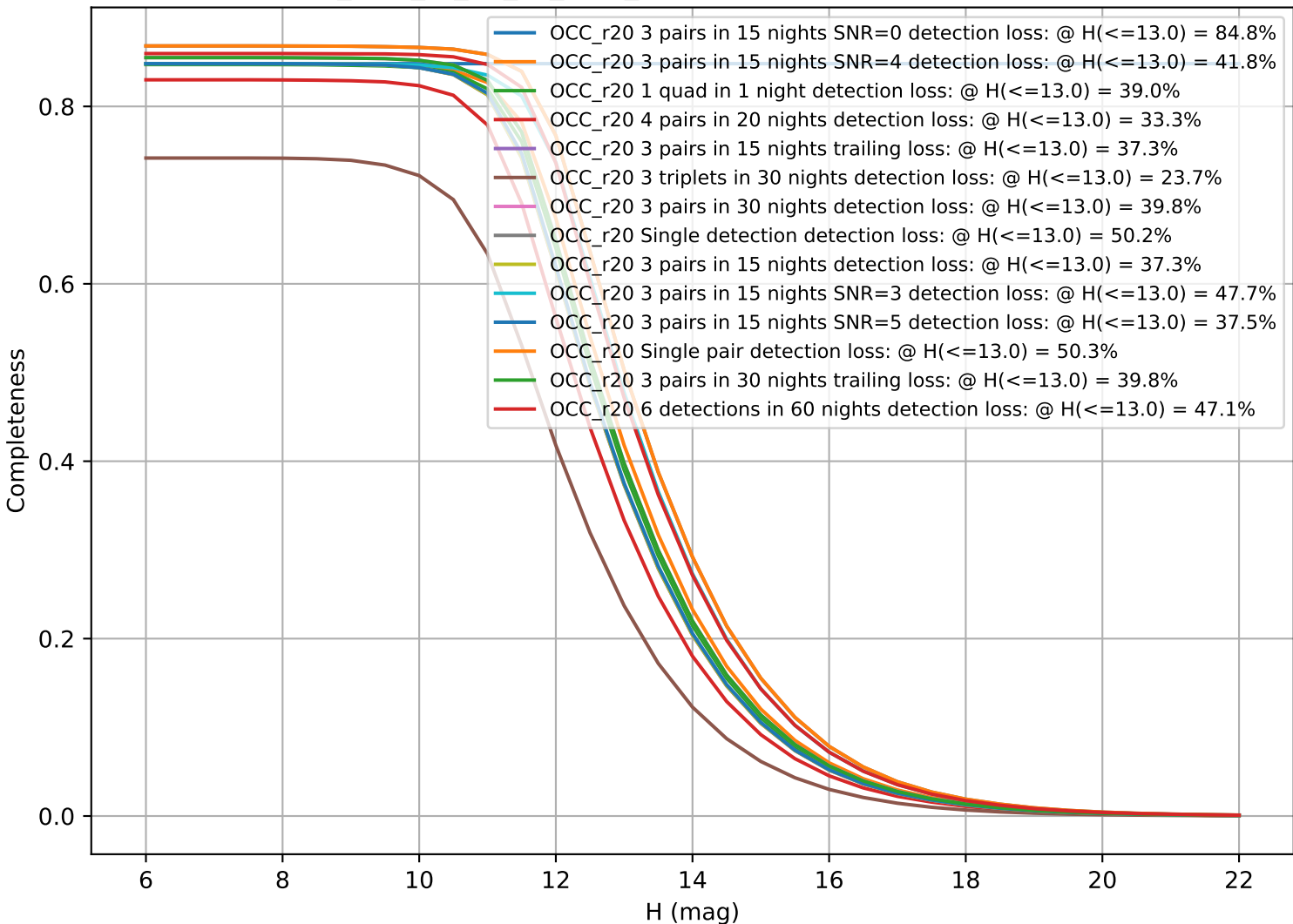
too_elab_r8_d2_gz_v3.4_10yrs: CumulativeCompleteness
