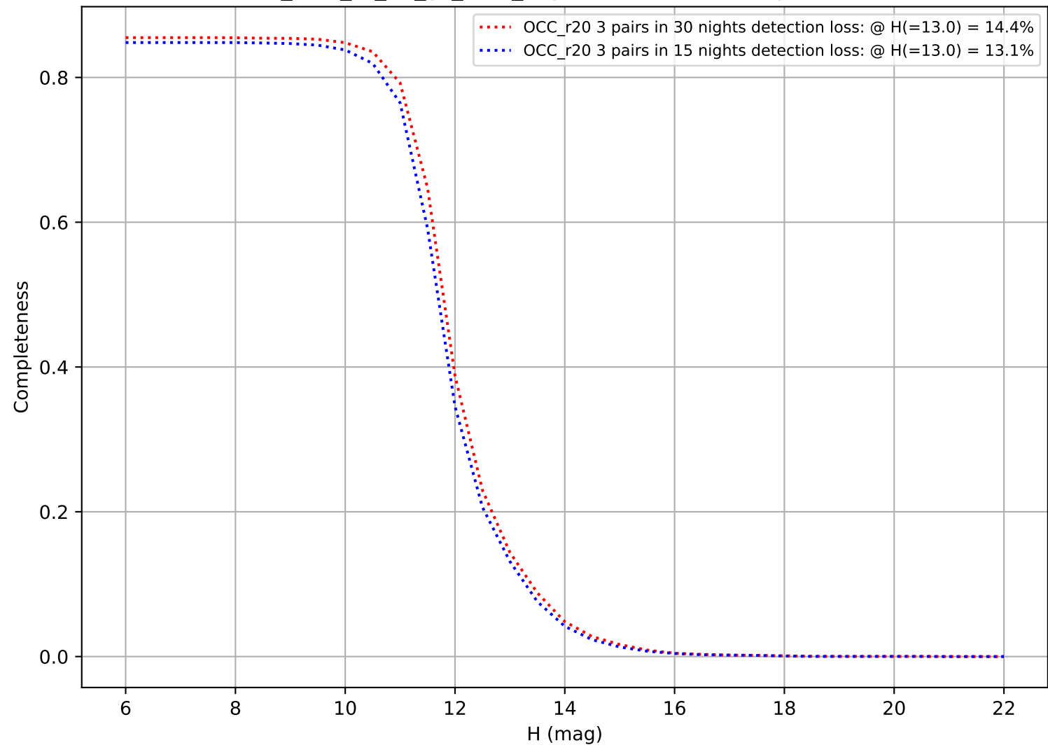
too_elab_r8_d2_gz_v3.4_10yrs: DifferentialCompleteness
