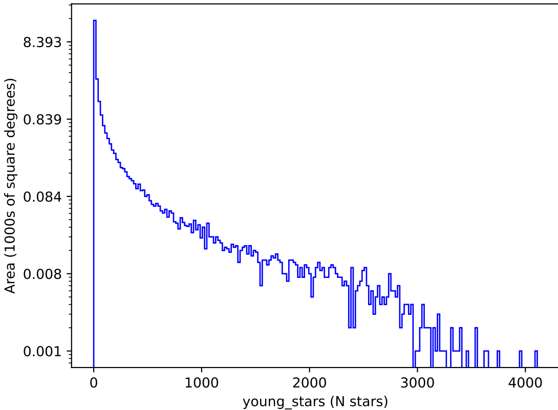
too_elab_r8_d2_gz_v3.4_10yrs : young_stars
