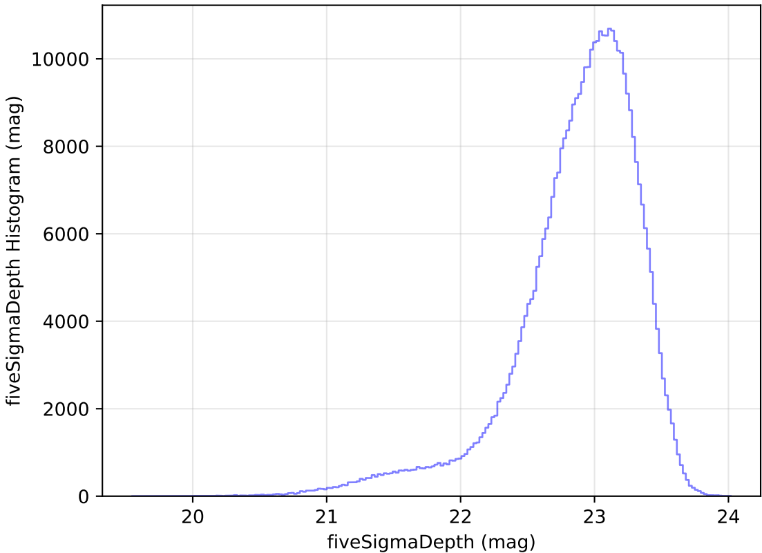
too_elab_r8_d2_gz_v3.4_10yrs z: fiveSigmaDepth Histogram
