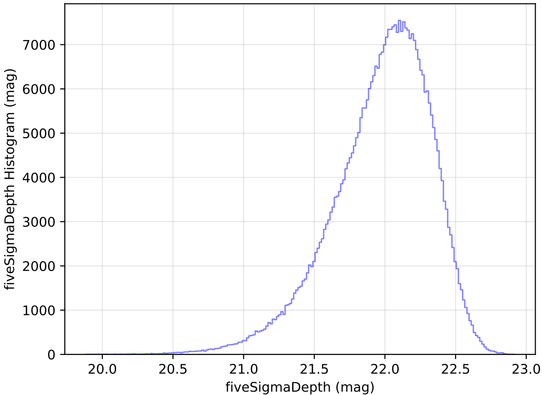
too_elab_r8_d2_gz_v3.4_10yrs y: fiveSigmaDepth Histogram
