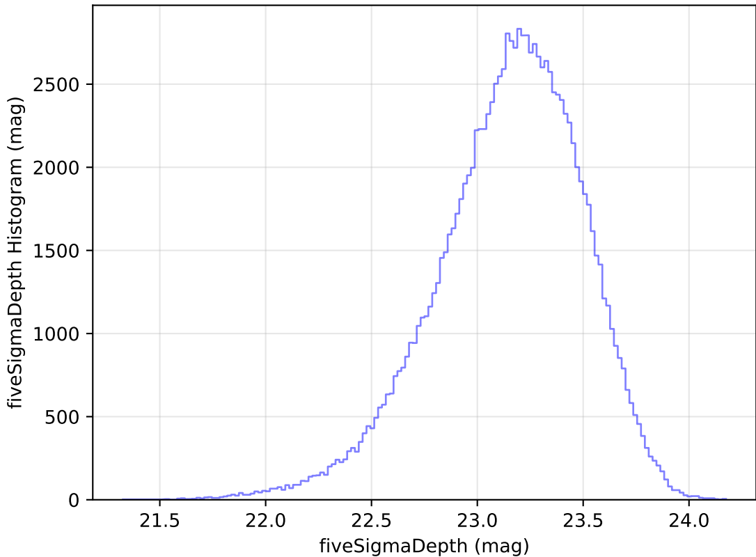
too_elab_r8_d2_gz_v3.4_10yrs u: fiveSigmaDepth Histogram
