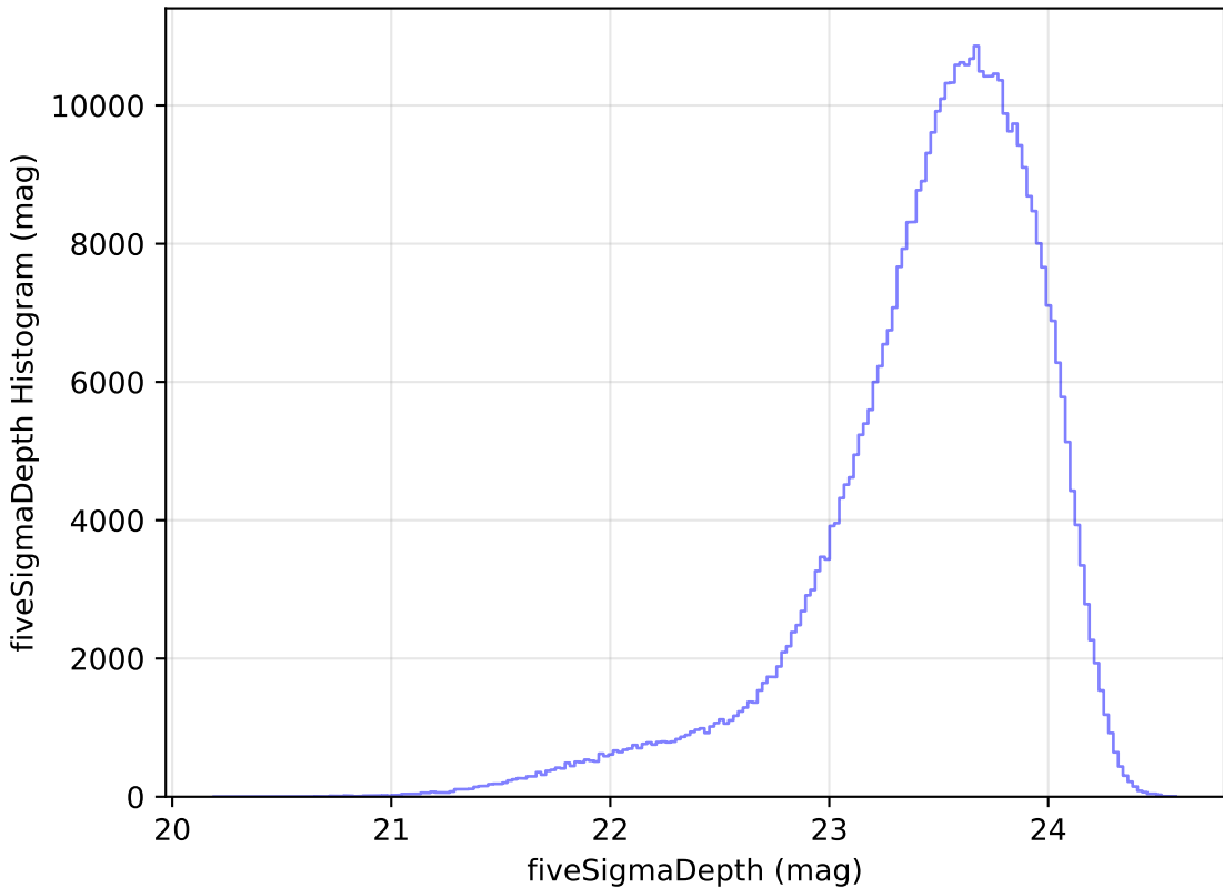
too_elab_r8_d2_gz_v3.4_10yrs i: fiveSigmaDepth Histogram
