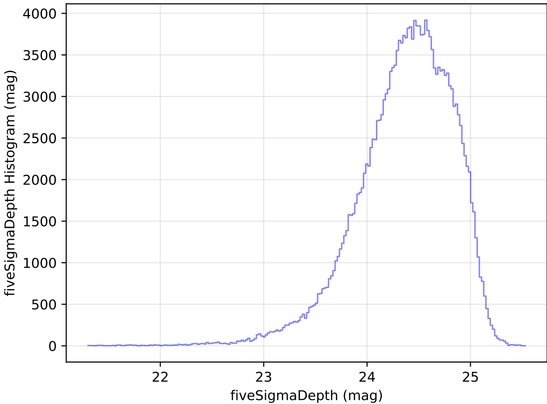
too_elab_r8_d2_gz_v3.4_10yrs g: fiveSigmaDepth Histogram
