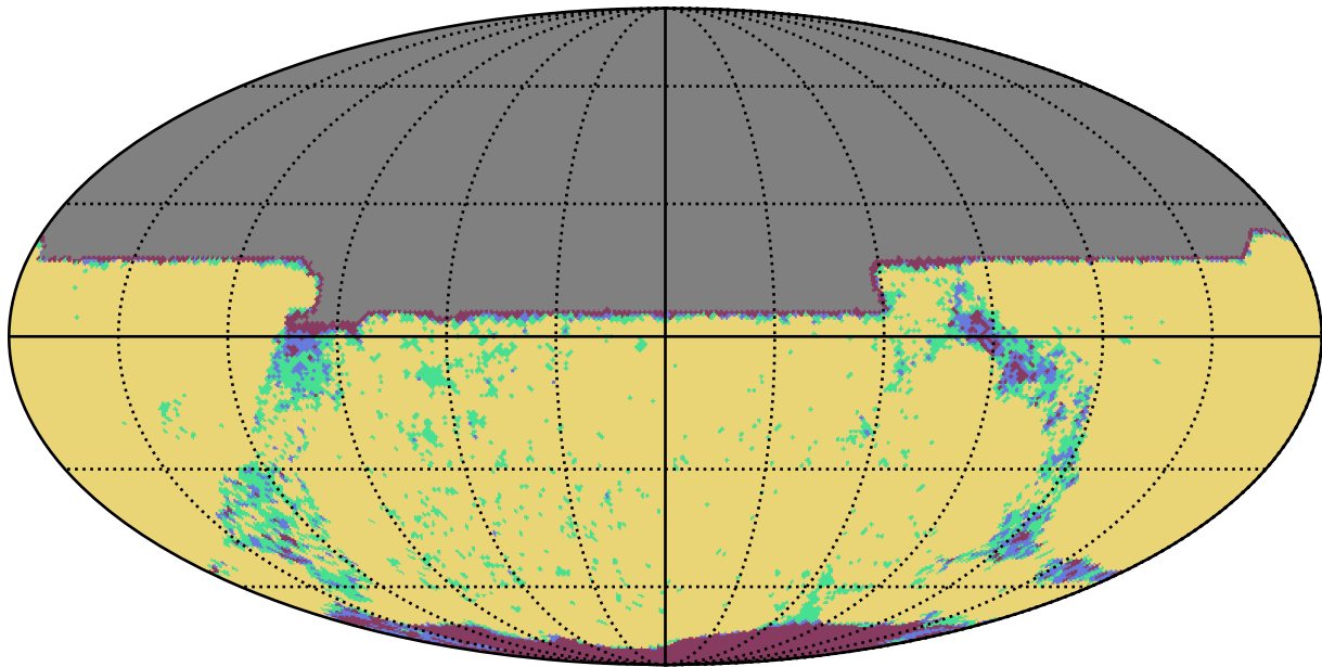
too_elab_r8_d2_gz_v3.4_10yrs y band: YearCoverage night
