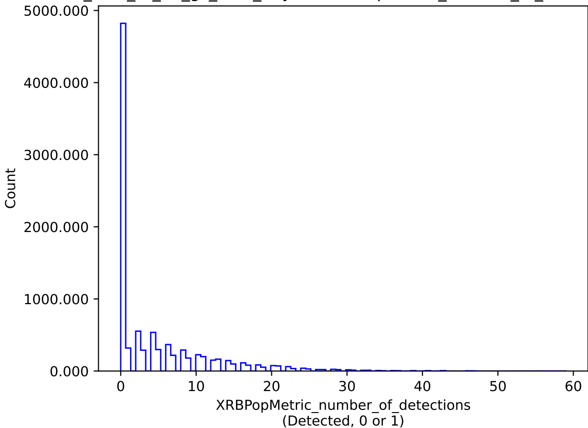
too_elab_r8_d2_gz_v3.4_10yrs : XRBPoMetric_number_of_detections
