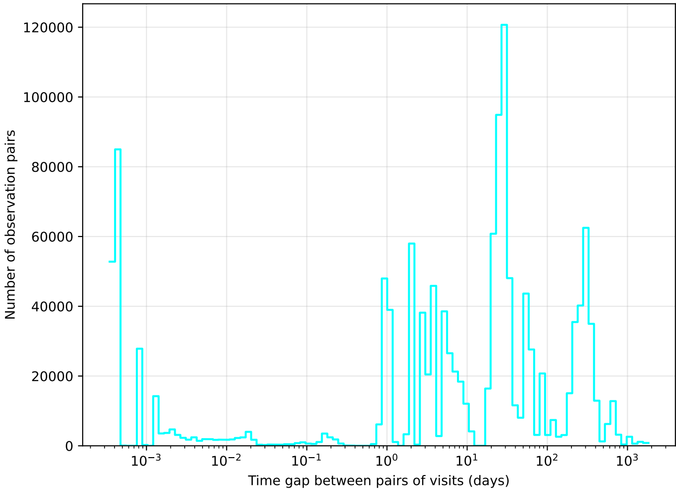
too_elab_r8_d2_gz_v3.4_10yrs u band: Tgaps observationStartMJD
