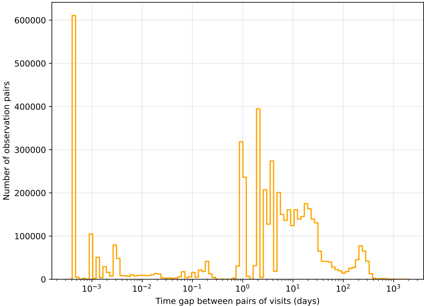
too_elab_r8_d2_gz_v3.4_10yrs r band: Tgaps observationStartMJD
