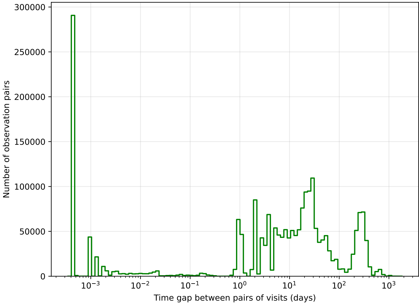
too_elab_r8_d2_gz_v3.4_10yrs g band: Tgaps observationStartMJD
