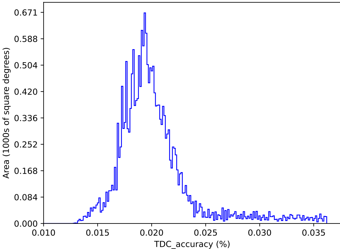
too_elab_r8_d2_gz_v3.4_10yrs : TDC_accuracy
