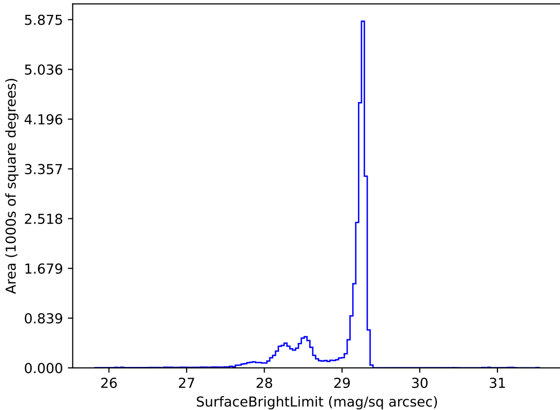
too_elab_r8_d2_gz_v3.4_10yrs z: SurfaceBrightLimit
