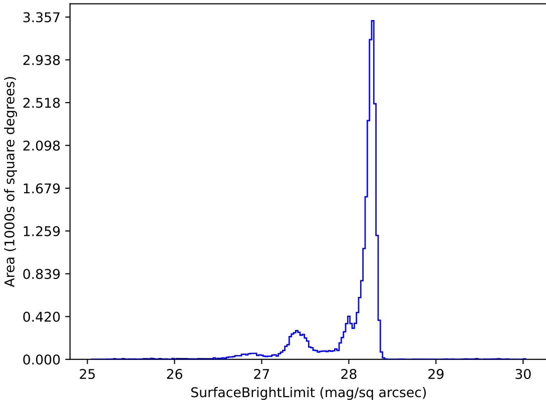
too_elab_r8_d2_gz_v3.4_10yrs y: SurfaceBrightLimit
