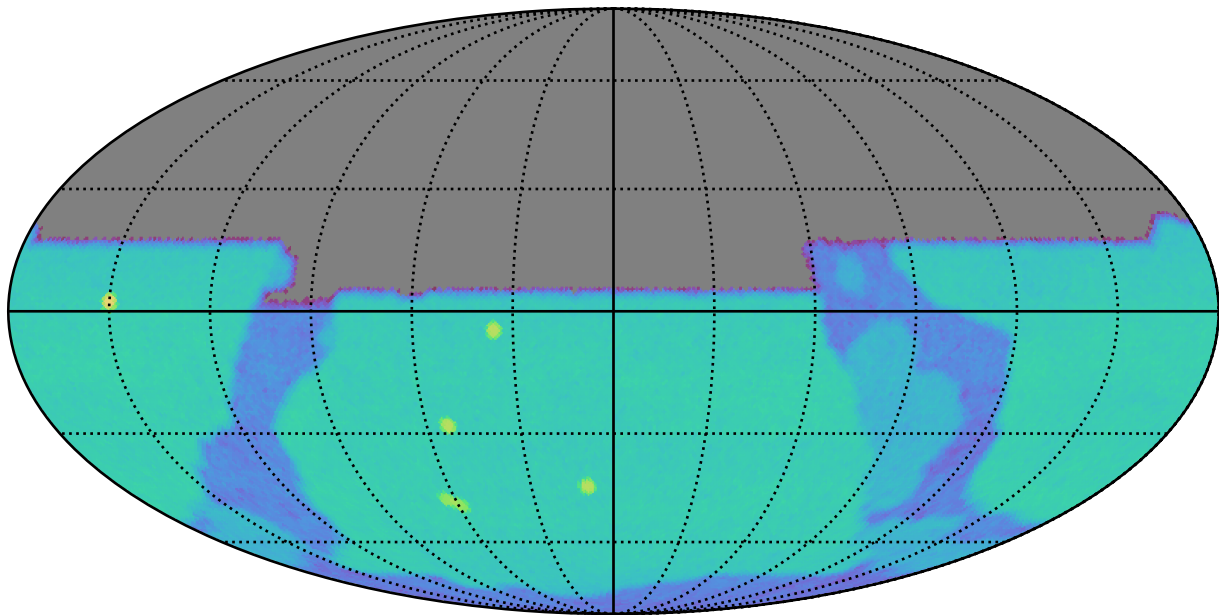
too_elab_r8_d2_gz_v3.4_10yrs u: SurfaceBrightLimit
