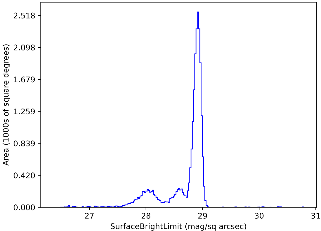
too_elab_r8_d2_gz_v3.4_10yrs u: SurfaceBrightLimit
