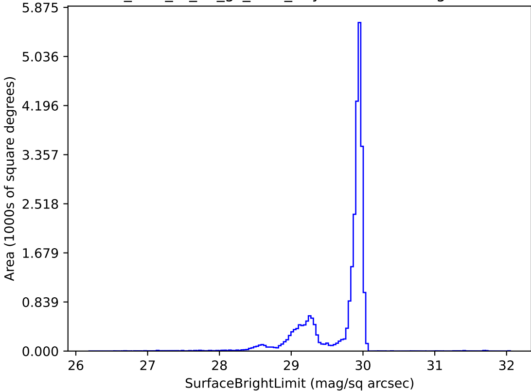
too_elab_r8_d2_gz_v3.4_10yrs i: SurfaceBrightLimit
