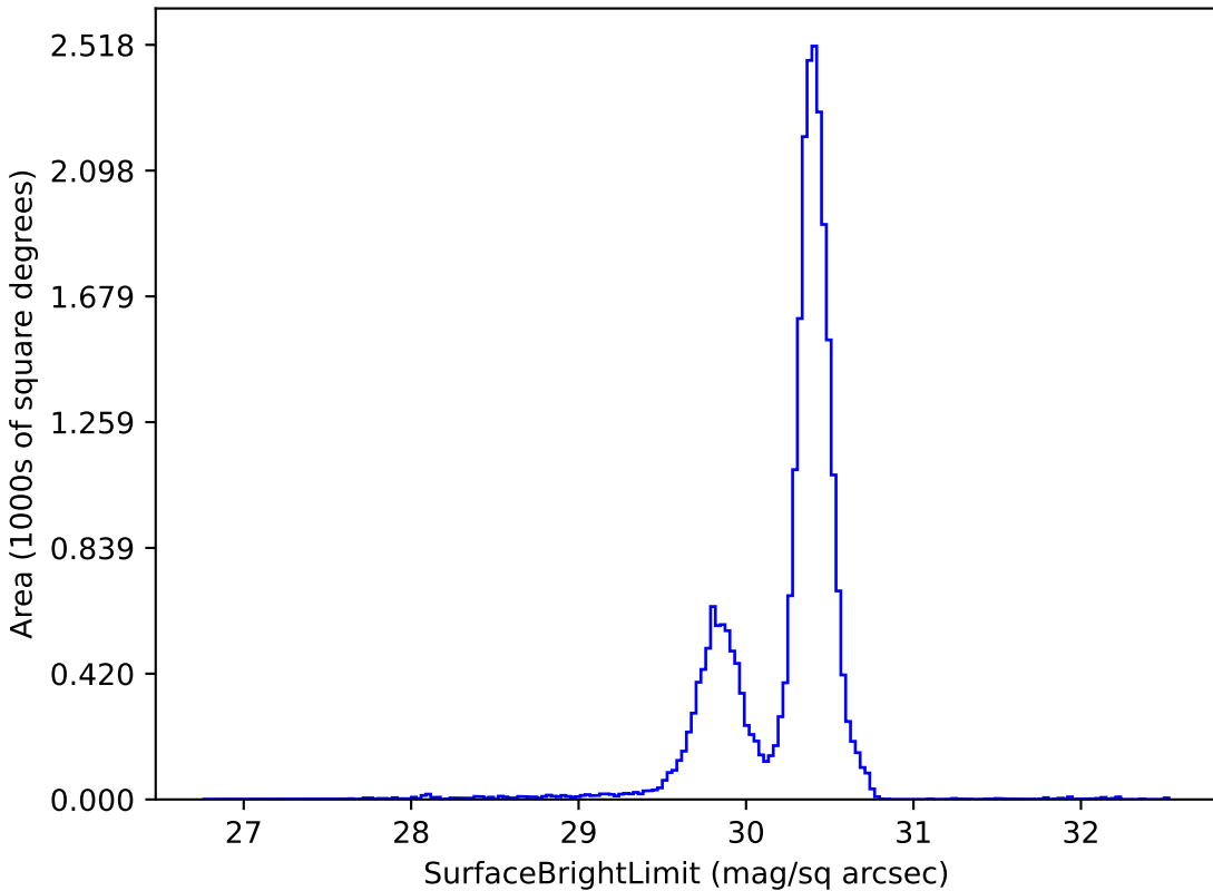
too_elab_r8_d2_gz_v3.4_10yrs g: SurfaceBrightLimit
