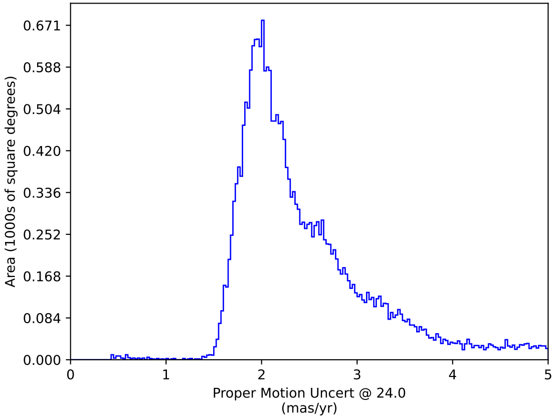
too_elab_r8_d2_gz_v3.4_10yrs : Proper Motion Uncert @ 24.0
