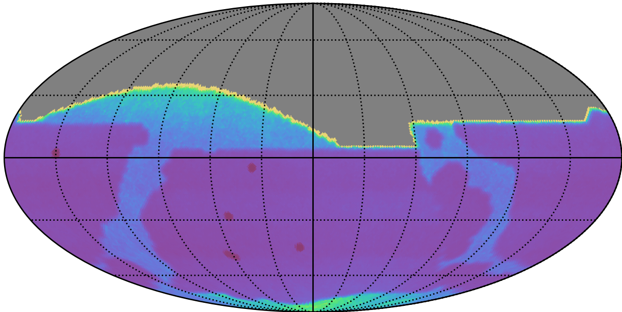
too_elab_r8_d2_gz_v3.4_10yrs : Proper Motion Uncert @ 20.5
