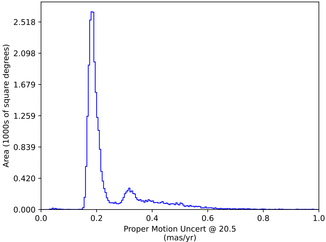
too_elab_r8_d2_gz_v3.4_10yrs : Proper Motion Uncert @ 20.5
