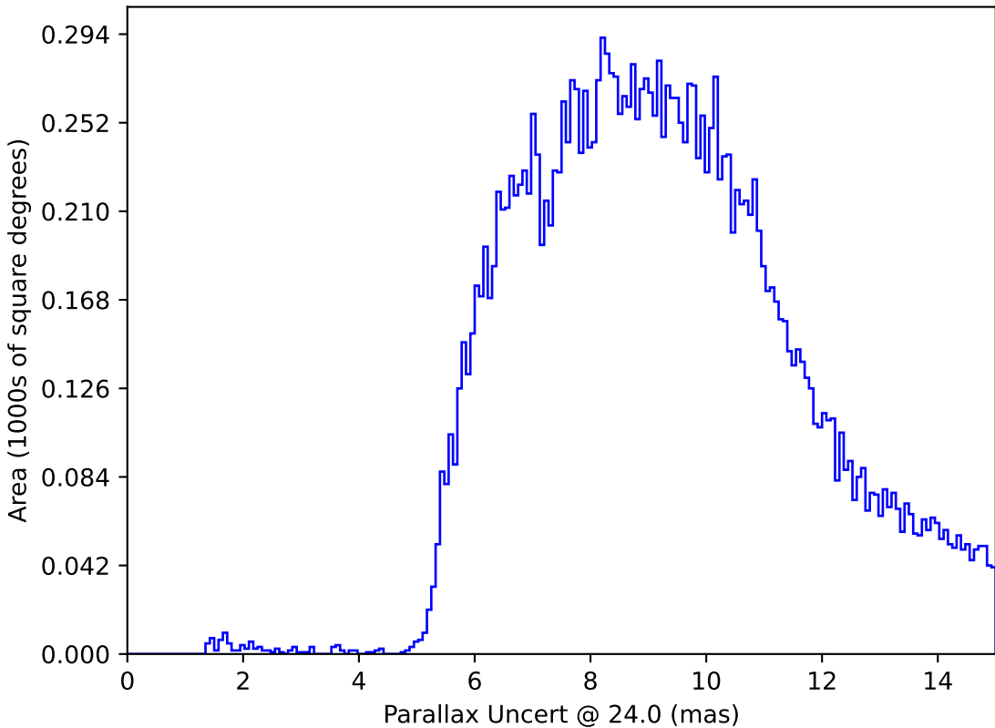
too_elab_r8_d2_gz_v3.4_10yrs : Parallax Uncert @ 24.0
