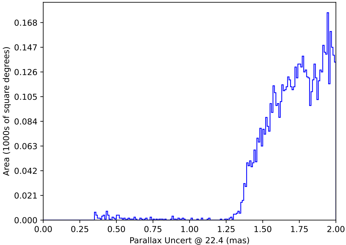
too_elab_r8_d2_gz_v3.4_10yrs : Parallax Uncert @ 22.4
