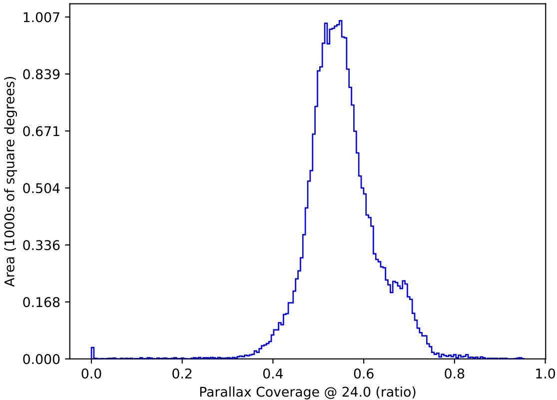
too_elab_r8_d2_gz_v3.4_10yrs : Parallax Coverage @ 24.0
