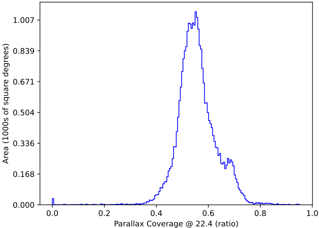
too_elab_r8_d2_gz_v3.4_10yrs : Parallax Coverage @ 22.4
