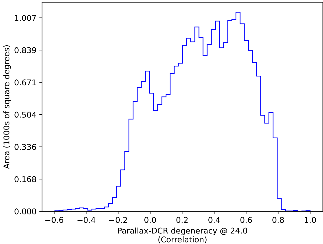
too_elab_r8_d2_gz_v3.4_10yrs : Parallax-DCR degeneracy @ 24.0
