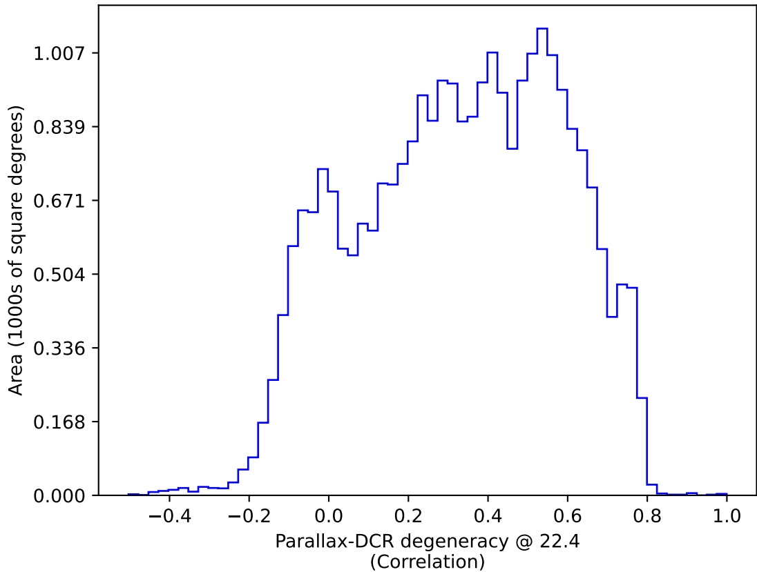
too_elab_r8_d2_gz_v3.4_10yrs : Parallax-DCR degeneracy @ 22.4
