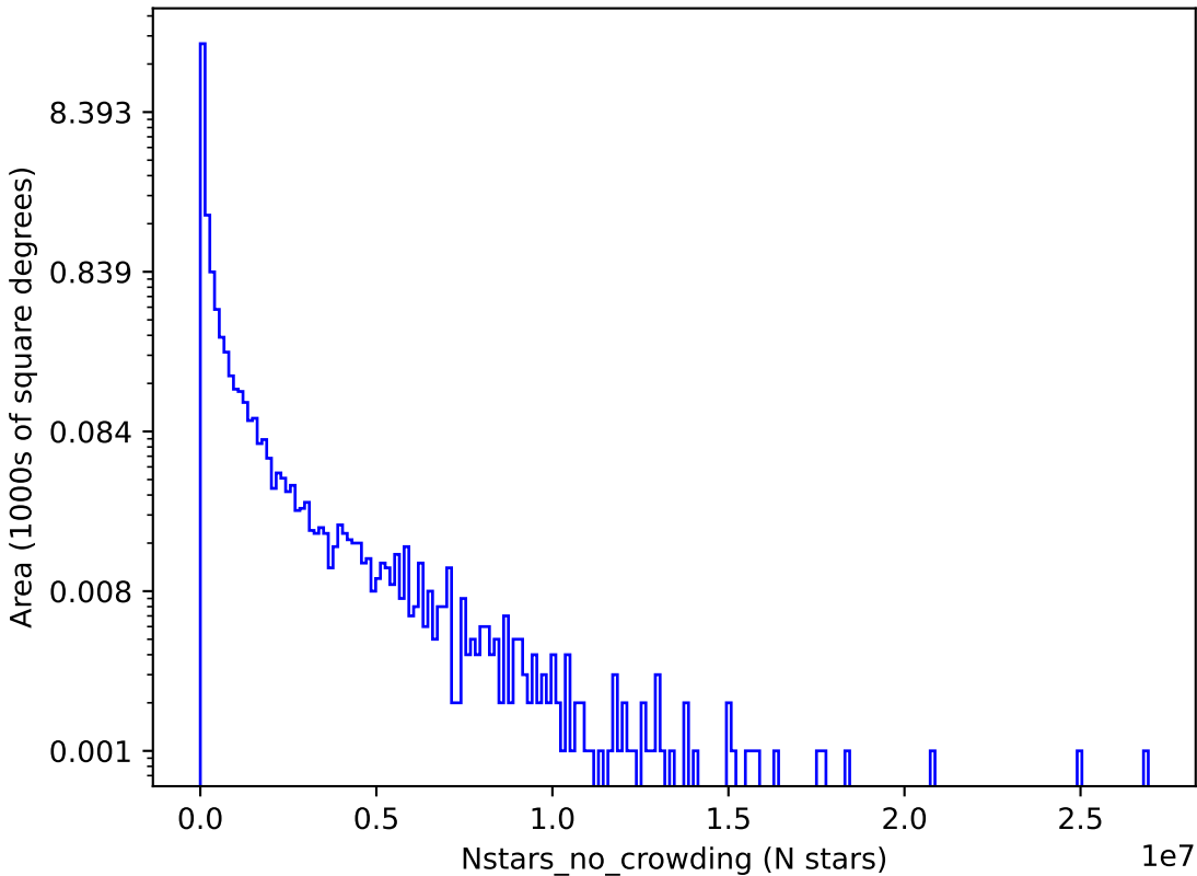
too_elab_r8_d2_gz_v3.4_10yrs z: Nstars_no_crowding
