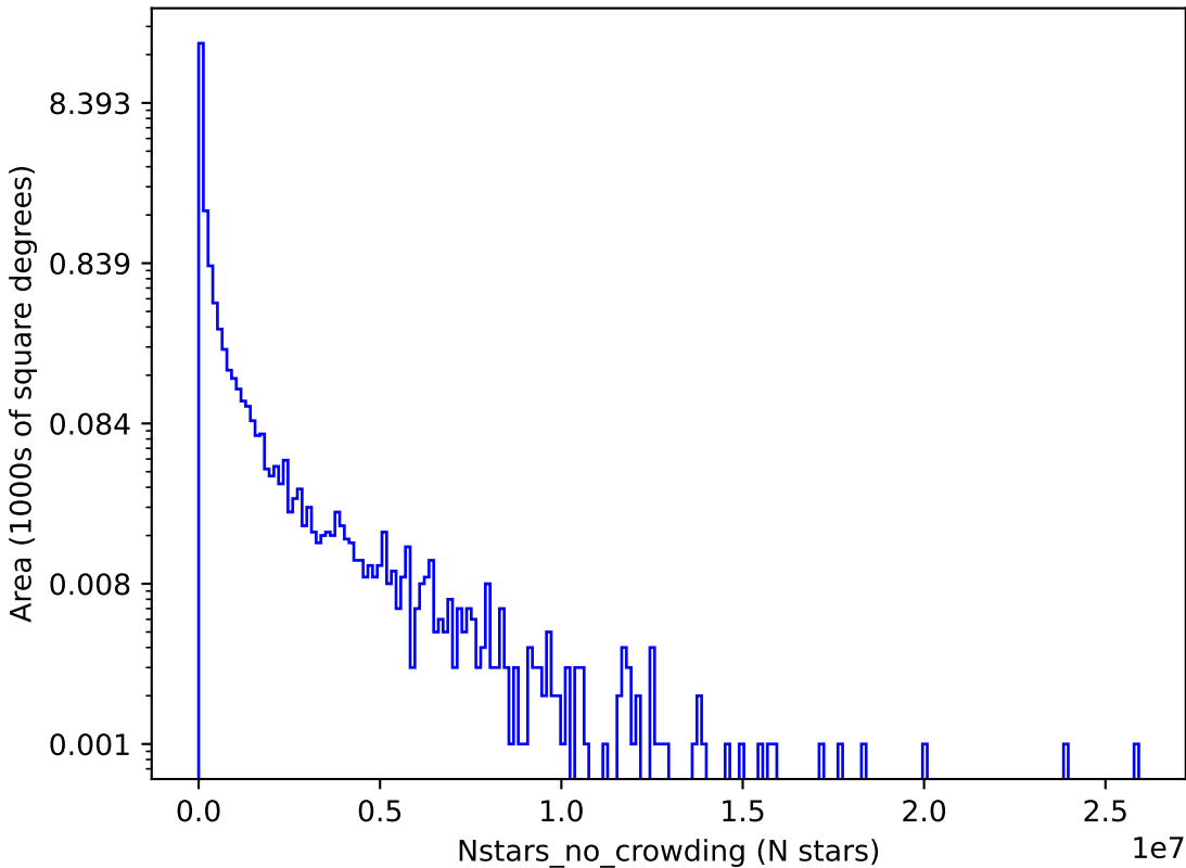
too_elab_r8_d2_gz_v3.4_10yrs y: Nstars_no_crowding
