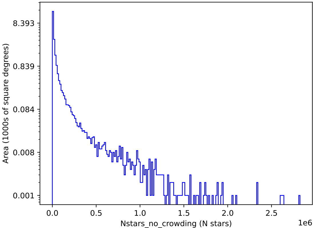
too_elab_r8_d2_gz_v3.4_10yrs u: Nstars_no_crowding
