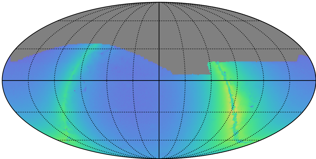
too_elab_r8_d2_gz_v3.4_10yrs r: Nstars_no_crowding
