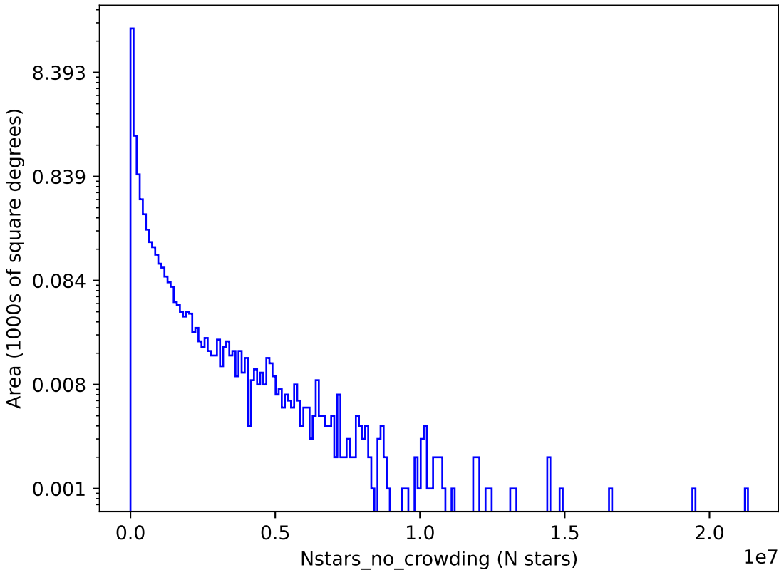
too_elab_r8_d2_gz_v3.4_10yrs r: Nstars_no_crowding
