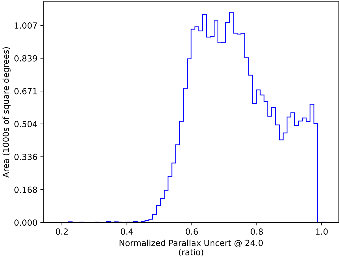
too_elab_r8_d2_gz_v3.4_10yrs : Normalized Parallax Uncert @ 24.0
