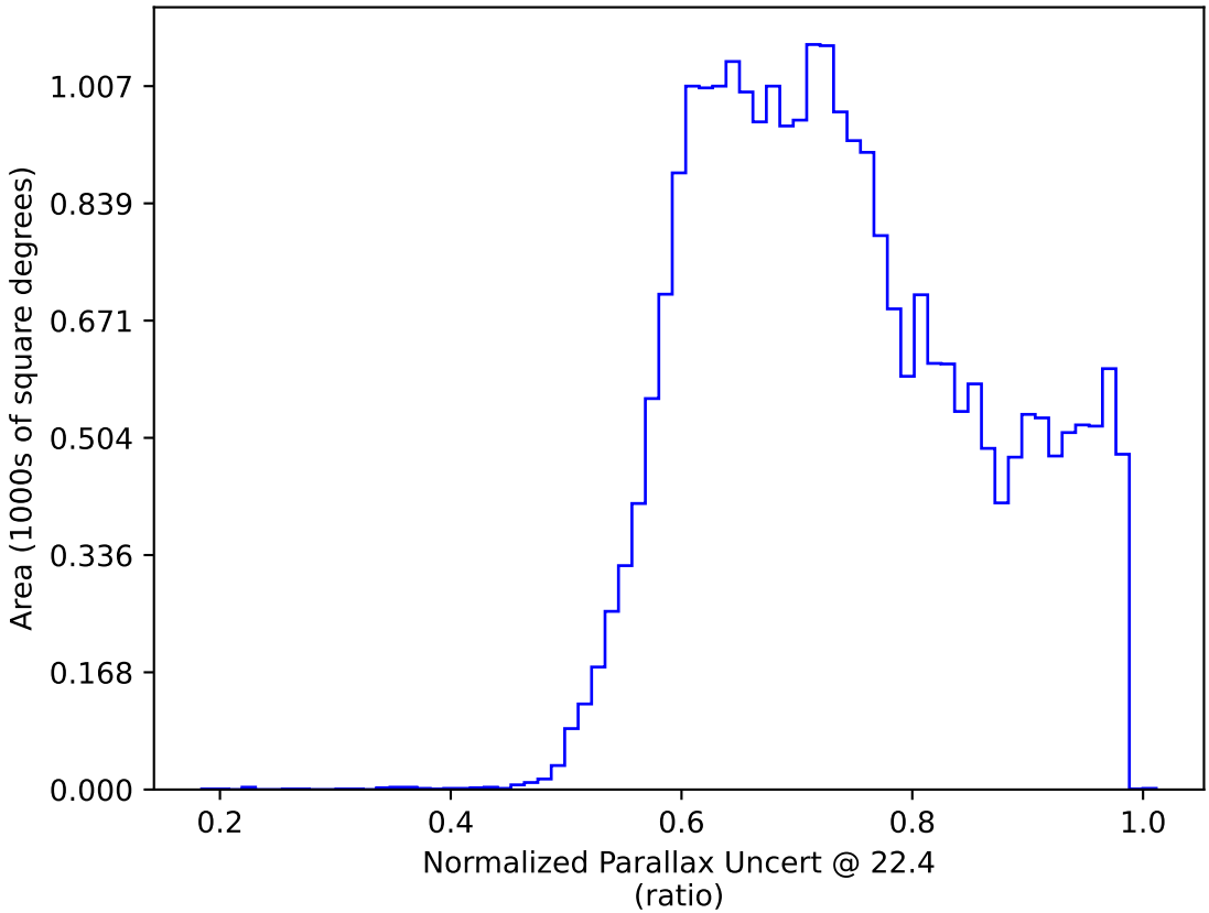
too_elab_r8_d2_gz_v3.4_10yrs : Normalized Parallax Uncert @ 22.4
